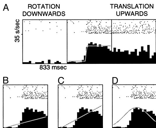
FIG. 5. Transition models fitted with the chi-square test. The step model ( A ) provides the best fit for this transition (Fig. 4 F ). The linear model ( B ), the straight line model ( C ), and the peak model ( D ) generated a higher chi-square value than the best-fitting model and were not selected for subsequent analysis.
