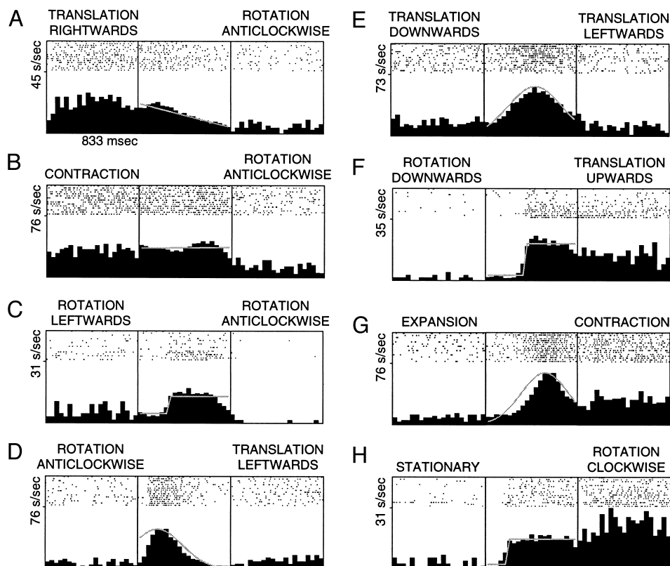
FIG. 4. Responses during transitions. Gray curves show the best-fit model. A : linear transition. The firing rate during the transition fits a line from the average firing rate of the rightward translation to the average firing rate of the anticlockwise rotation. B : straight-line model. The firing rate of the cell could not be predicted by the two contiguous flow fields; instead it was constant throughout the transition and toward the end the firing rate dropped to the firing rate of the successive stimulus. C : step model. The response profile was characterized by a sudden change in the middle of the transition followed by a decrease in the firing rate at the end. D : peak model. The firing rate gradually increased and then decreased during the transition. The firing rate at the peak of the transition was higher than during the response to the two contiguous stimuli. E : direction tuning. Another example of a peak transition, which shows a strong response of the cell in the middle of the transition, corresponding to a specific direction of translation (approximately -45^\circ ). F : transition with a stationary random-dot pattern in the middle. Transitions with opposite or near-opposite from- and to-stimuli often fit the step model. In this case, the first half of the transition consisted of a decelerating downward motion and the second part of an accelerating upward motion. G : another case of transition with a stationary pattern in the middle. In this case, a peak-shaped response suggests that the cell was responsive to contraction, but at low speeds, and not responsive to expansion. H : acceleration. The clockwise rotation gains speed gradually from the initial stationary random-dot pattern. Unlike the previous cell, this cell was not strongly sensitive to speed. The firing rate suddenly increased as the speed reached a threshold for the cell and it remained constant during the rest of the transition and the following clockwise rotation.
