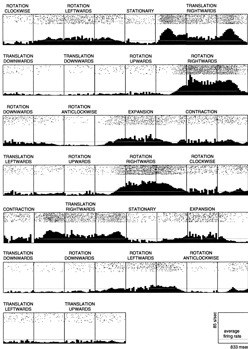
FIG. 2. Movie sequence from a transition-tuning test. The histograms (read from left to right, top to bottom) represent the complete sequence of stimuli presented to an MST cell 20 times, which included two presentations of each cardinal flow-field and 27 transitions. Histograms corresponding to cardinal-flow fields are labeled. Non-labeled histograms refer to transitions, which are defined by two adjacent stimuli. The cell responded with a similar firing rate to each of the two presentations of the same flow field. The response profile during the transitions depended in several cases on the stimuli defining the transitions (the to- and from-stimuli), but the responses obtained during the cardinal flow-fields did not always predict the response during the transitions. The transitions from a stationary pattern to a rightward translation and then to a downward translation offer an example. The peak in the transition to rightward translation can be explained as an effect of speed tuning: the speed of the rightward translation gradually increased and the peak corresponded to a low-speed translation. In the following transition, the rightward translation gradually shifted to a downward rotation by changing the angle of translation (in the middle, the transition is a -45^\circ translation). The peak may reflect a preference of the cell for an intermediate direction.
