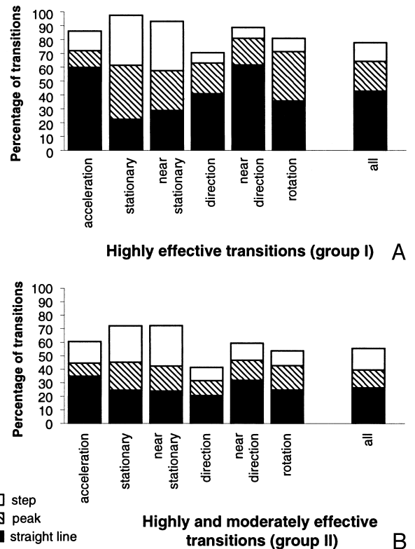
FIG. 8. Distribution of transition models among nonlinear transitions. In both the highly effective ( A ) and effective ( B ) groups, a higher percentage of step models fit the stationary and near-stationary transitions (Fig. 4F). In the first group, a high-density of peak models was associated with stationary, near-stationary, and rotation types. During acceleration and near-direction transitions, straight-line models were more frequently fit than on average.
