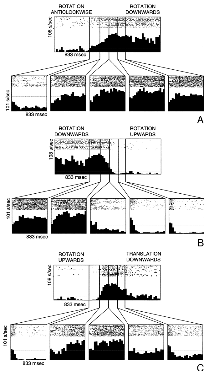
FIG. 9. Temporal-independence test in a single cell, with three transitions tested (all of them fit the peak model). For each section, the top panel shows the response obtained during the transition-tuning test. The bottom panel shows the responses of the cell to cardinal (the from- and to-stimuli, first and last histograms , respectively) and linear-combination flow fields ( middle three histograms ) that replicated flow-field patterns shown during the transition, in correspondence to the vertical lines. During the transition the flow-field patterns appeared only for a frame interval; in the cardinal and linear-combination flow fields, the same pattern was presented continuously for 833 ms. The vertical lines show the response of the cell during the transition to the flow-field patterns presented in the bottom panels . The horizontal lines show the average firing rate of the transition-tuning test in the top panels and the average firing rate elicited by the linear-combination flow field stimuli in the bottom panels . A : the gradual initial increase and final decrease in the firing rate during the transition was replicated in the temporal-independence test. B : a reversal of direction of the flow field caused a rather sharp decrease in the firing rate after an initial increase. The same pattern was present in the temporal-independence test. The initial response in the last three histograms in the bottom panel was caused by sustained response to the preceding stimuli. C : in the third transition the match between the transition pattern and the responses to the cardinal and linear-combination flow fields was not as precise as in the first two cases, although the overall peak pattern of the transition was maintained.
