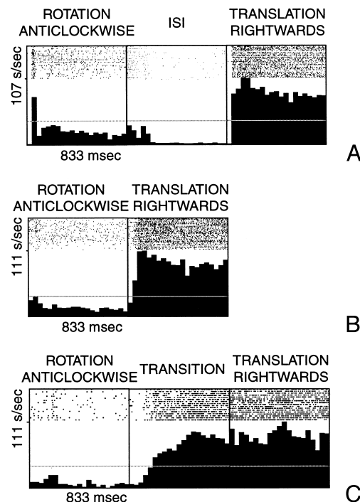
FIG. 1. Temporal structure of the response of a medial superior temporal (MST) cell to the same stimuli in different temporal contexts. The horizontal gray line represents the average firing rate across all conditions for a given test. A : flow-field stimuli separated by an interstimulus interval (ISI). The cell was responsive to rightward translation. The peak in the first stimulus was a nonspecific response to the stimulus onset and was present in all conditions (not shown). B : continuous presentation of flow fields (without ISI). At the onset of the new stimulus, the dots in the flow-field pattern suddenly changed direction. The tuning of the cell was preserved, but the nonspecific peak at the stimulus onset disappeared. C : stimuli interleaved with transitions. Again, we did not observe any change in the tuning of the cell. During the transition, the anticlockwise component decreased linearly as the rightward translation component increased and the firing rate gradually increased.
